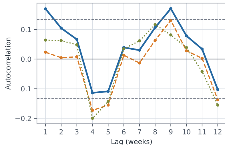
c. Unique one-step residual ACF
