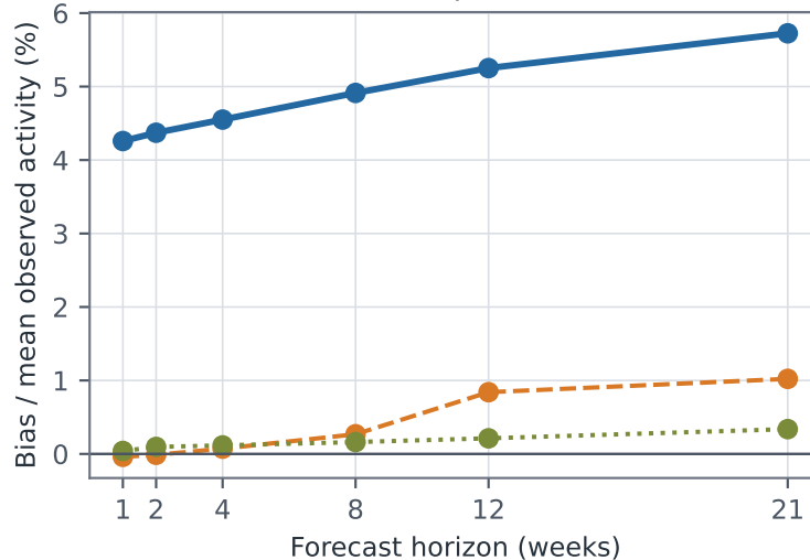
b. Normalised prediction bias
