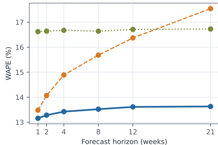
a. Cumulative path WAPE
